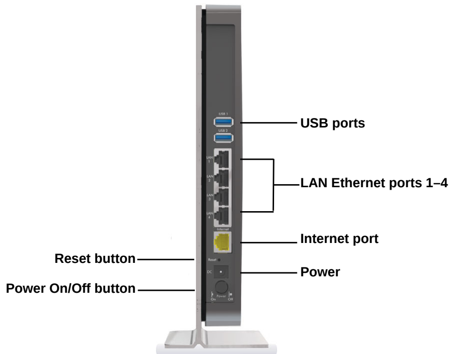
Figure 3. Router, rear view
