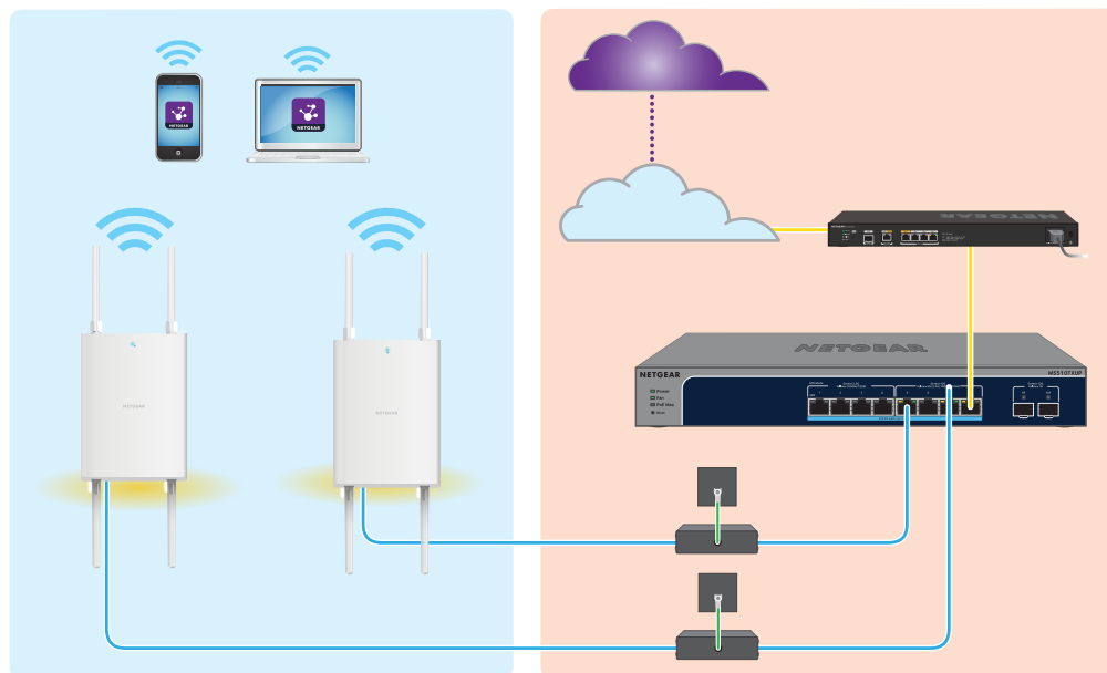
Figure 5. Set up the access point in a NETGEAR Insight configuration
