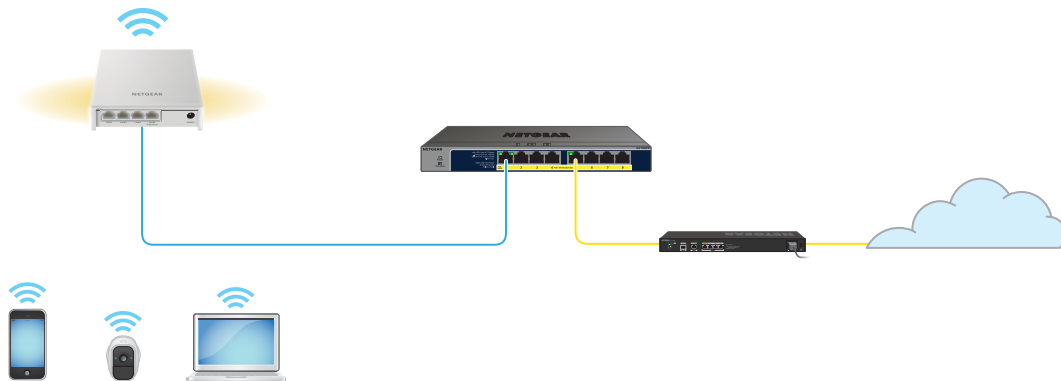
Figure 5. Set up the access point with a PoE connection to your network
