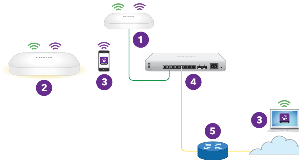
Figure 11. Connect the node to a wired root
