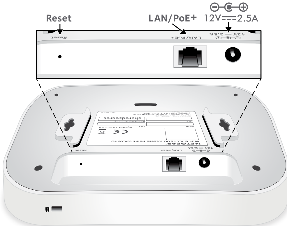
Figure 2. Hardware interfaces of the access point
