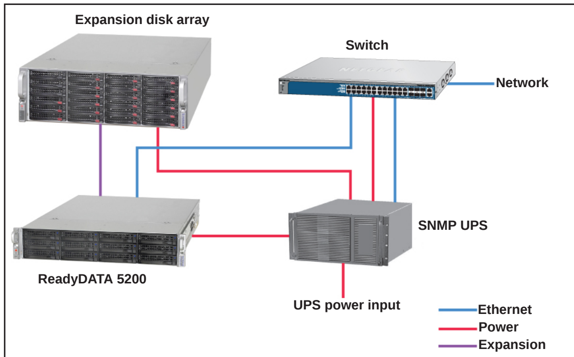
Figure 10. ReadyDATA and expansion disk array with a UPS managed over SNMP
