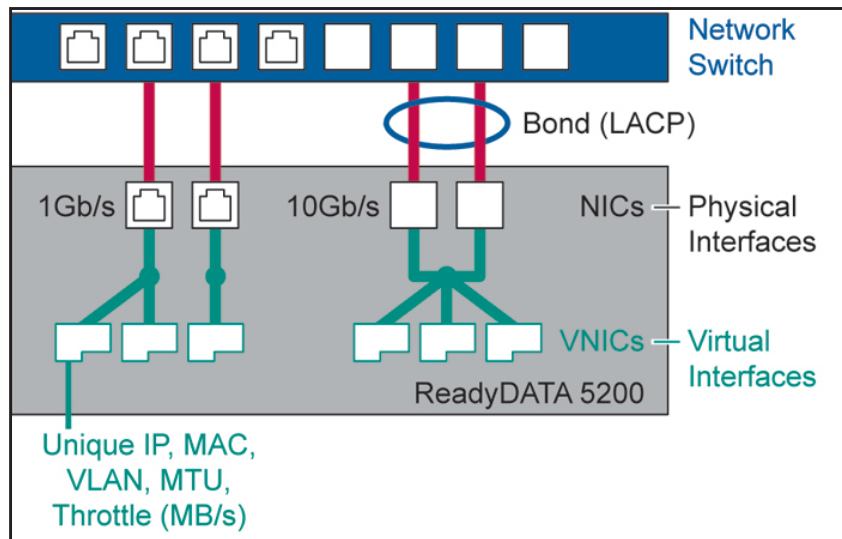
Figure 3. VNICs in a ReadyDATA Network Configuration
