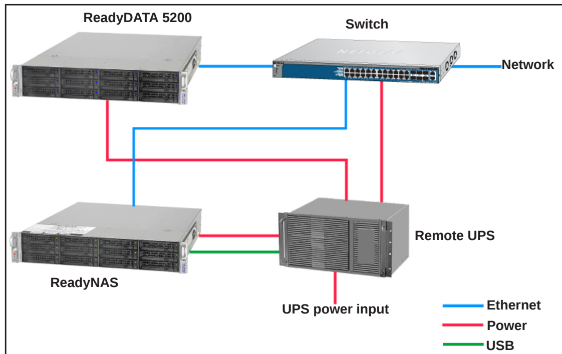
Figure 12. ReadyDATA with a UPS managed remotely over a remote ReadyNAS
