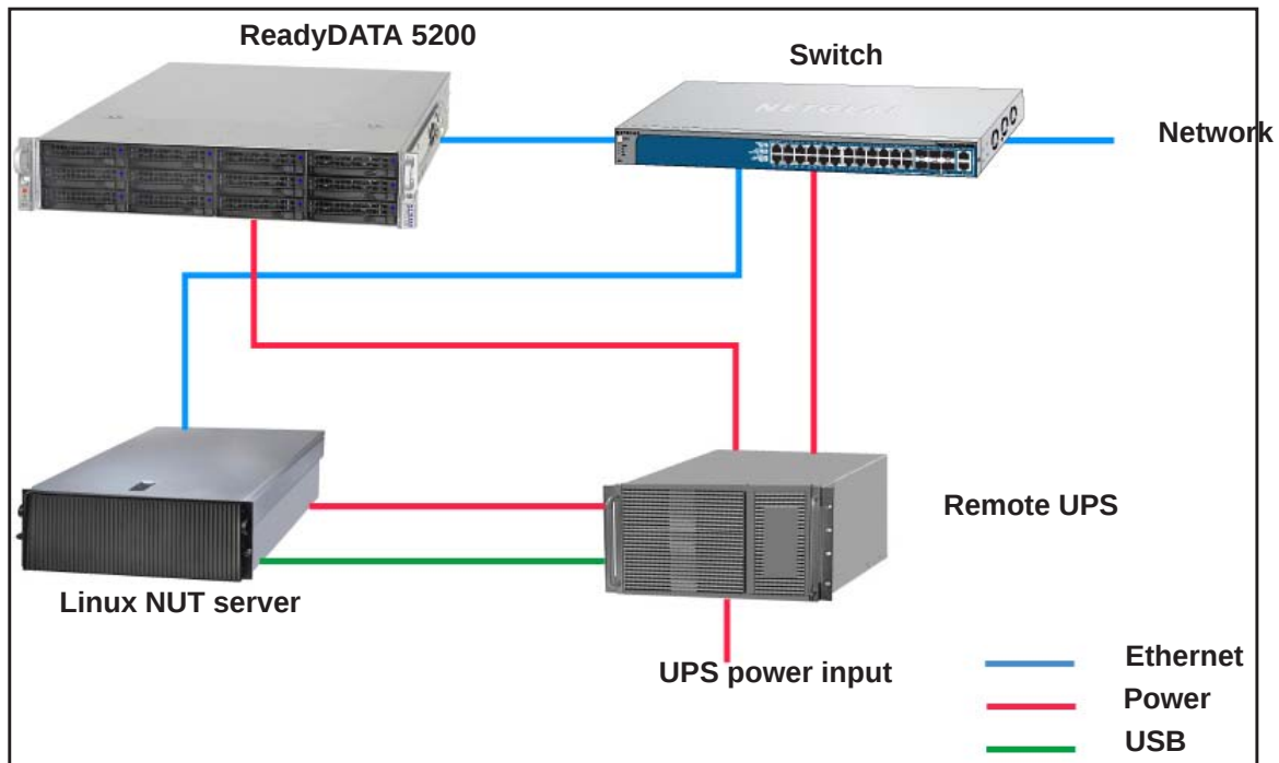
Figure 11. ReadyDATA with a UPS managed remotely over a Linux NUT server
