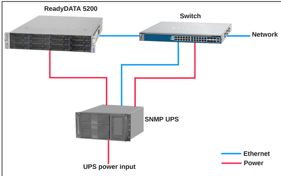
Figure 8. ReadyDATA with a UPS managed over SNMP
