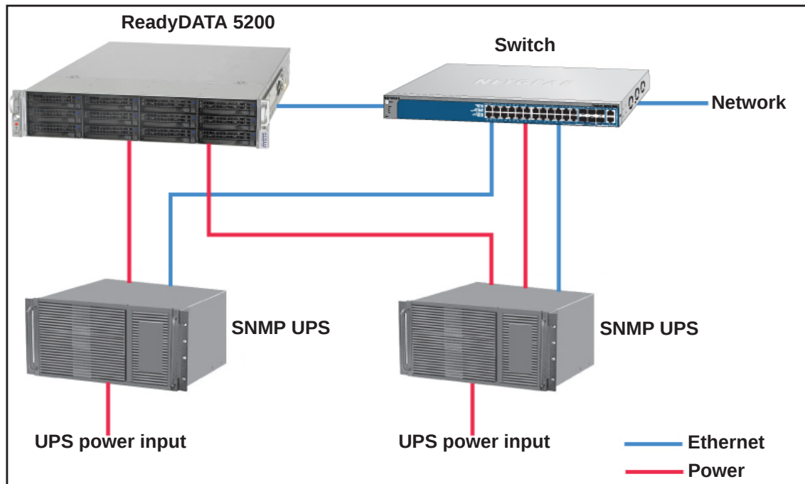
Figure 9. ReadyDATA with dual UPS devices managed over SNMP
