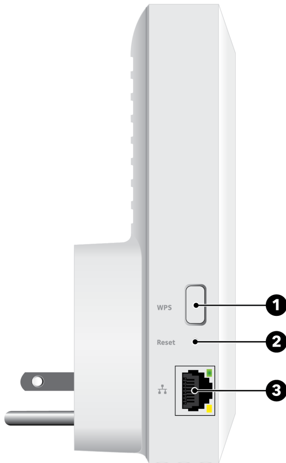
Figure 3. Back panel
