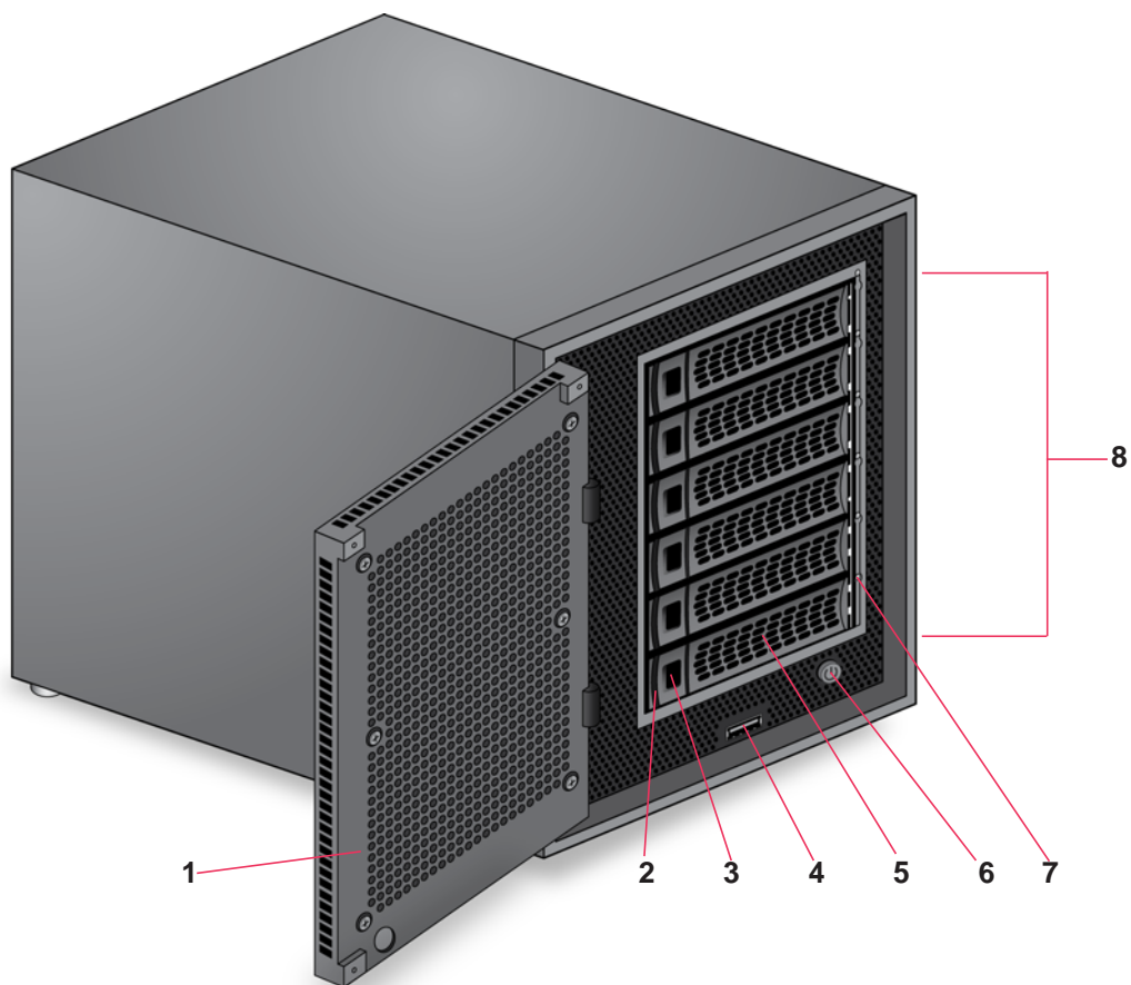
Figure 26. ReadyNAS 716X drive bays
