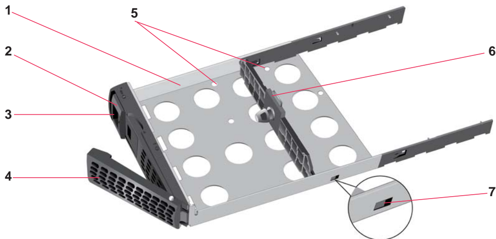
Figure 31. Standard disk tray
