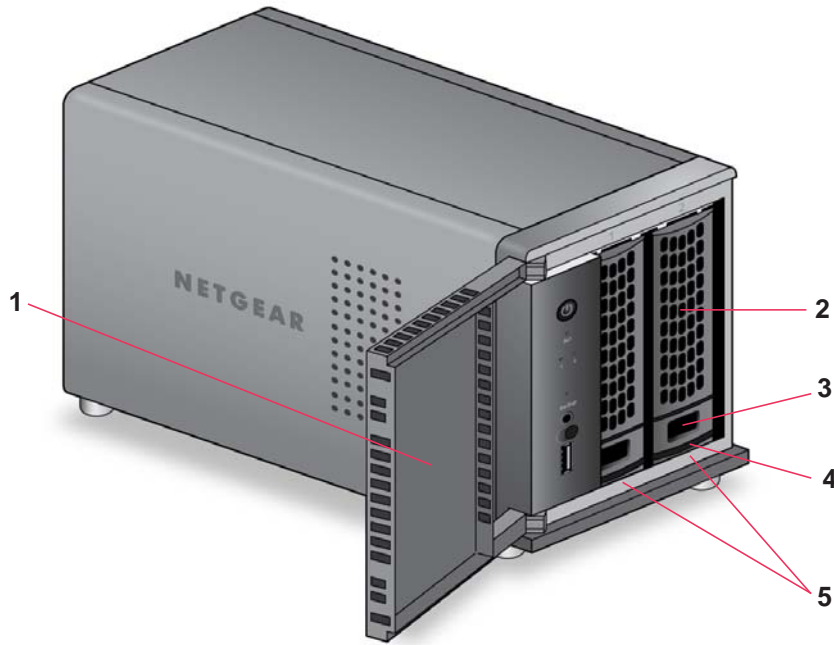
Figure 14. ReadyNAS 312 drive bays
