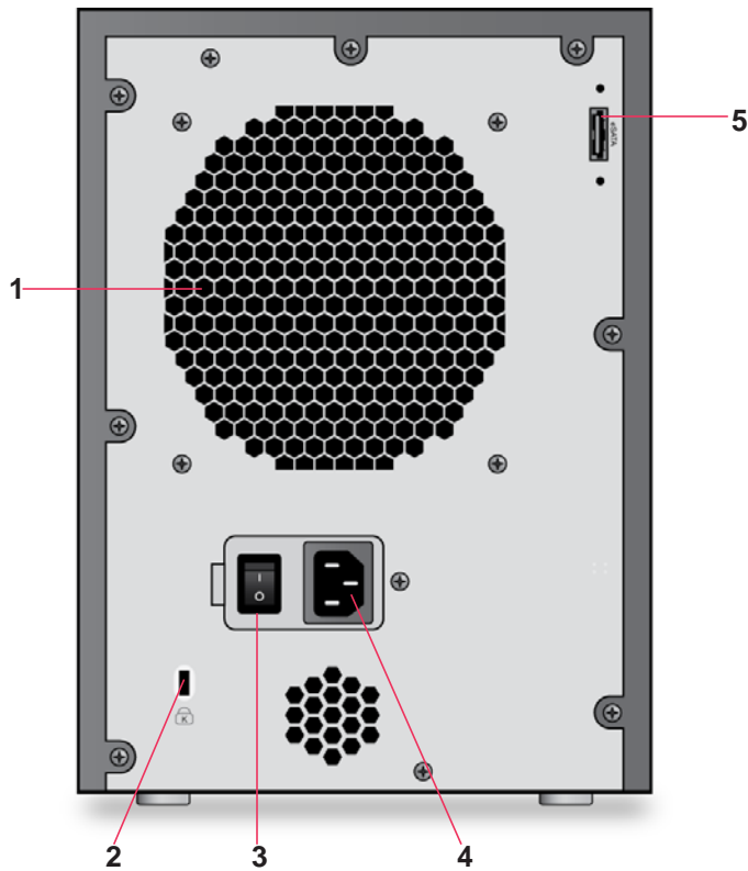
Figure 30. EDA 500 rear panel
