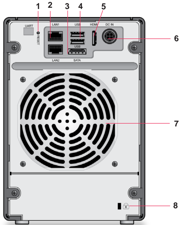
Figure 18. ReadyNAS 314 rear panel
