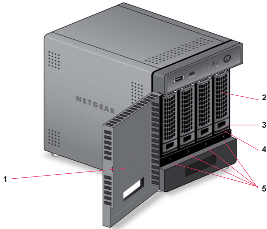
Figure 17. ReadyNAS 314 drive bays
