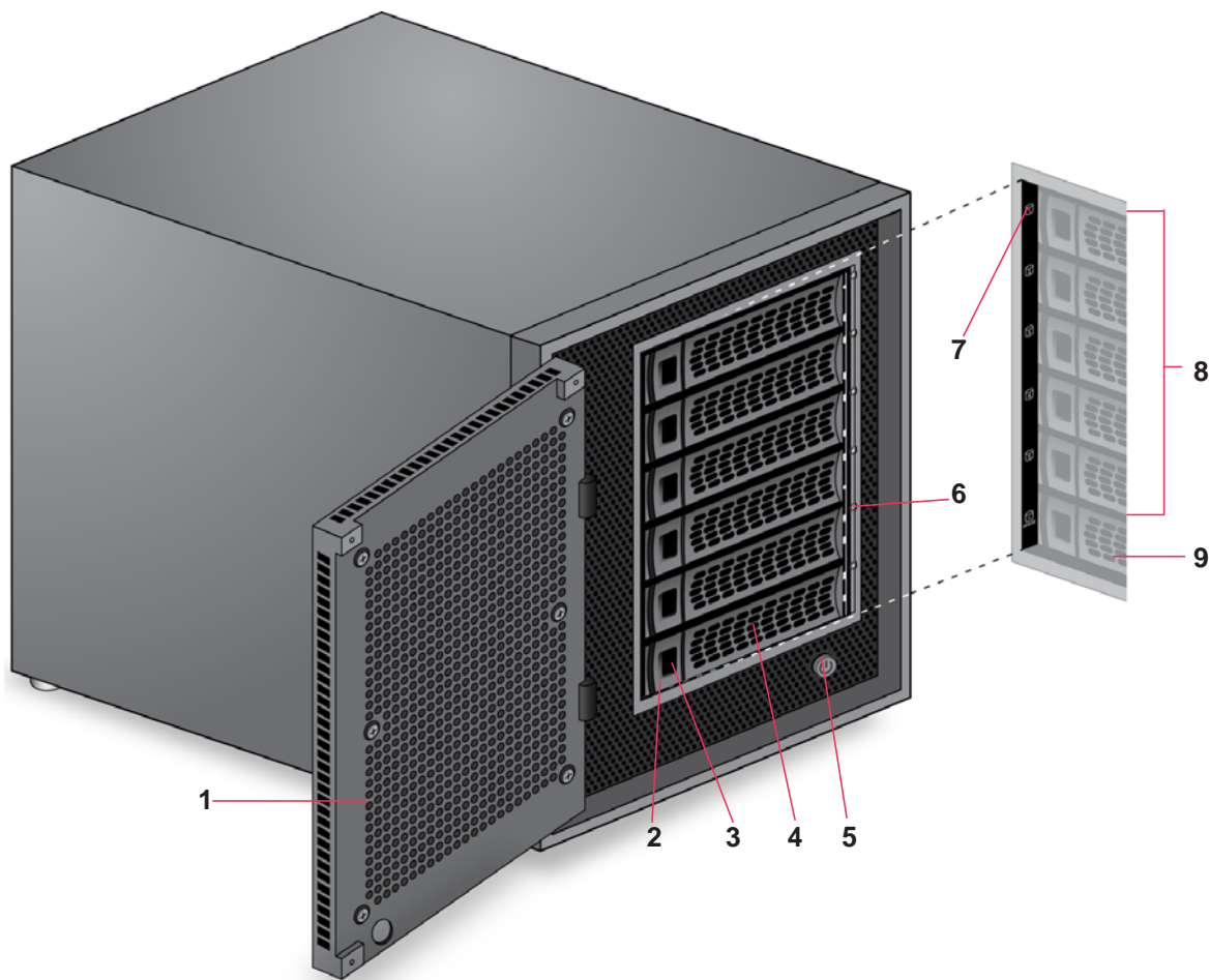
Figure 29. EDA 500 drive bays
