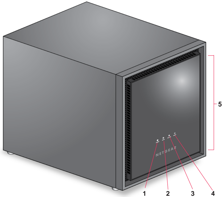
Figure 28. EDA 500 front and side panels
