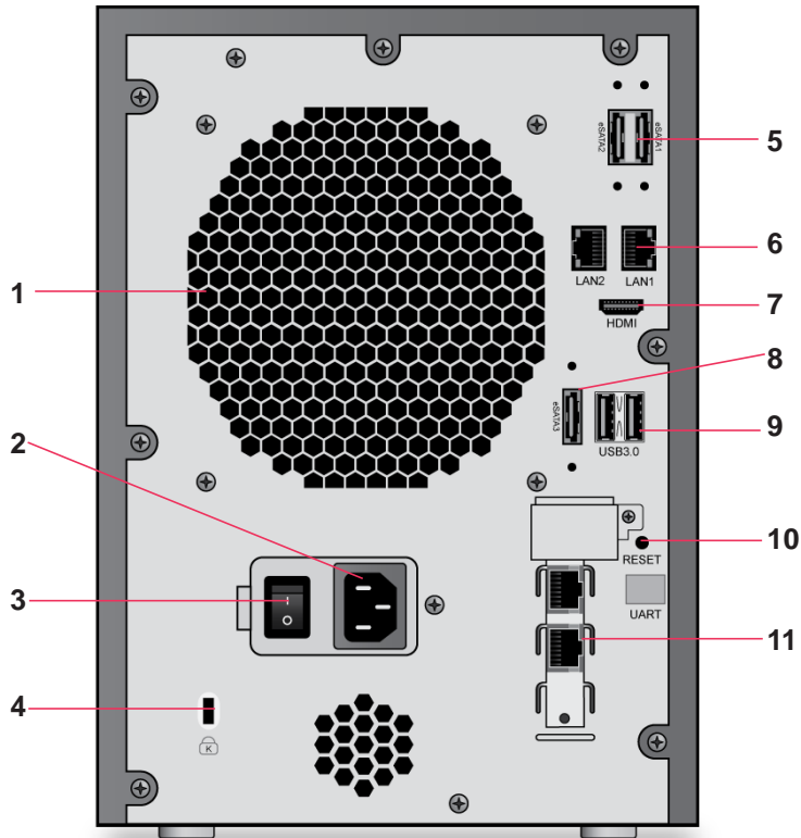
Figure 27. ReadyNAS 716X rear panel
