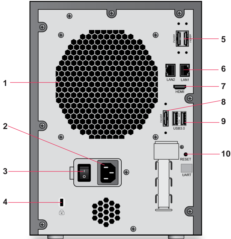
Figure 24. ReadyNAS 516 rear panel
