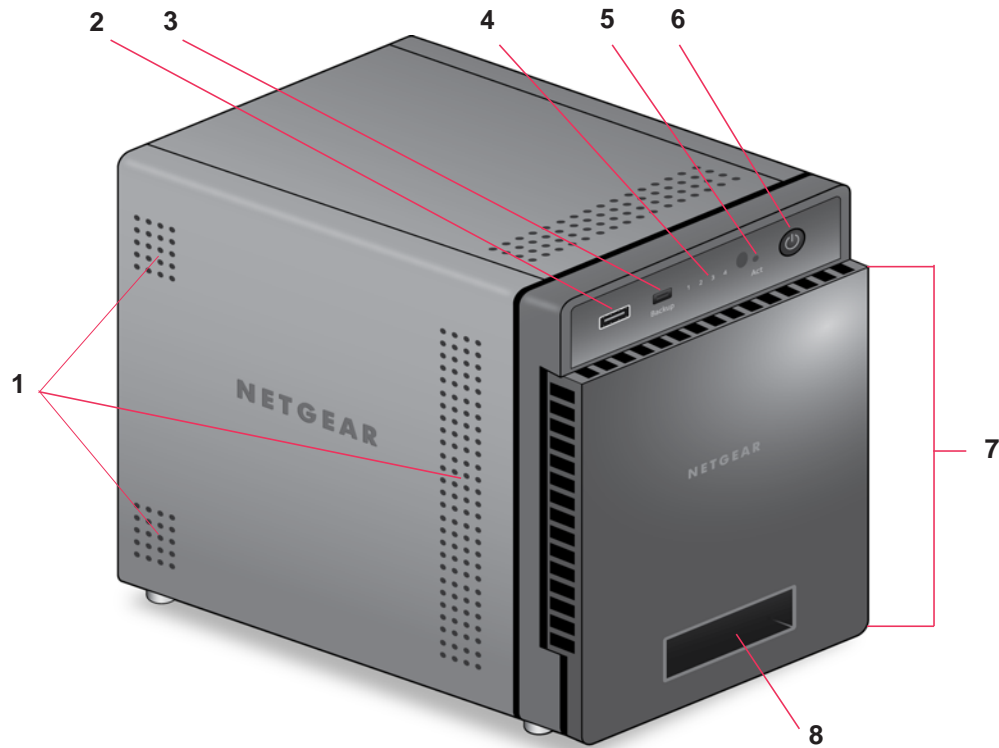
Figure 10. ReadyNAS 204 front and side panels
