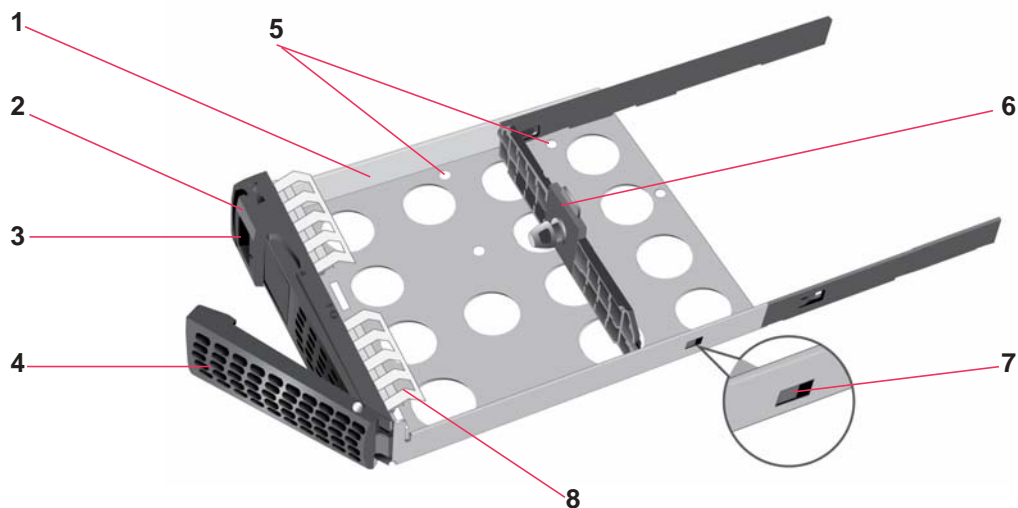
Figure 32. EDA 500 disk tray
