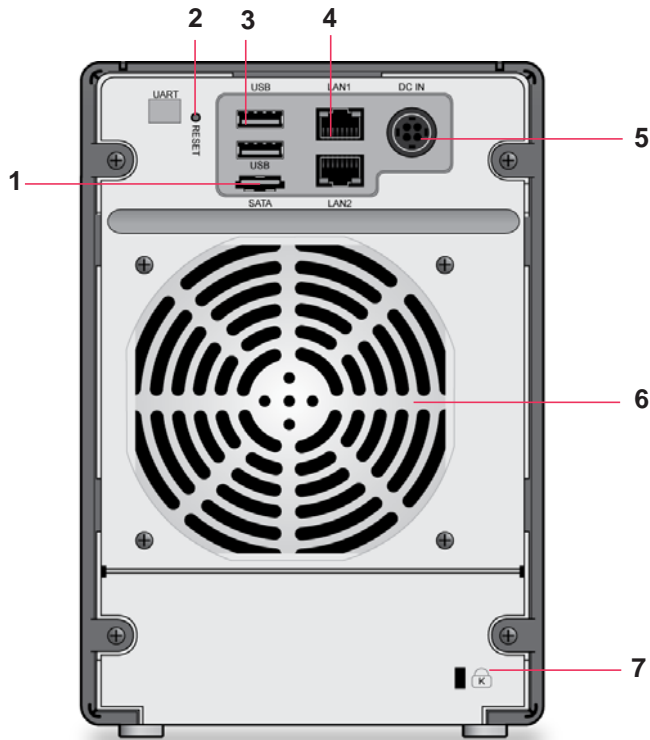
Figure 12. ReadyNAS 204 rear panel
