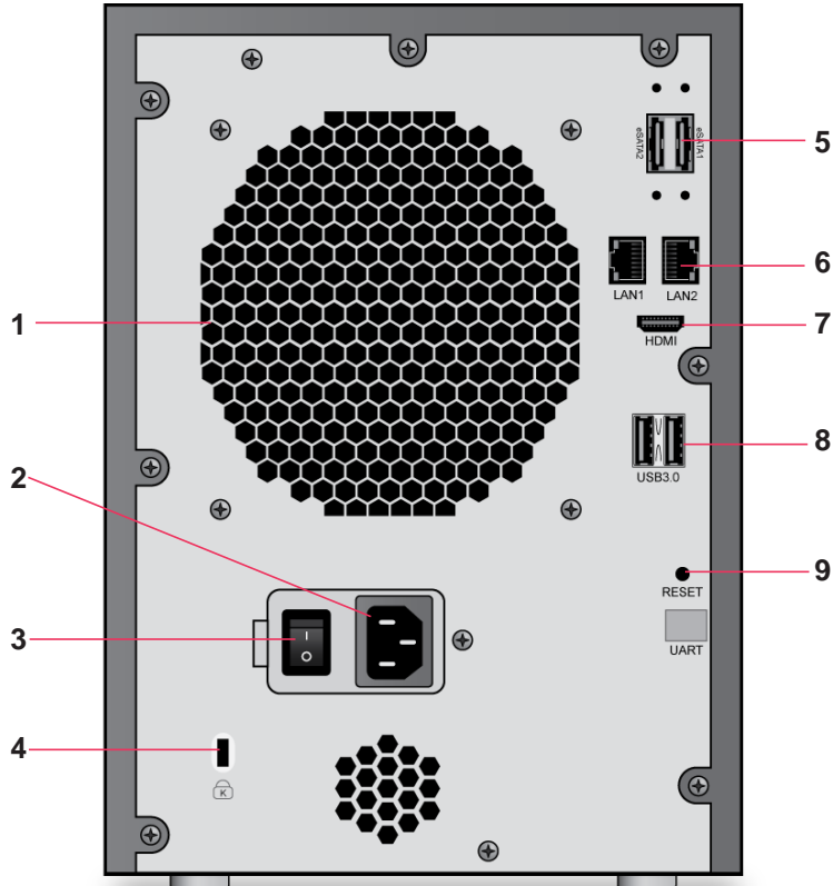
Figure 21. ReadyNAS 316 rear panel
