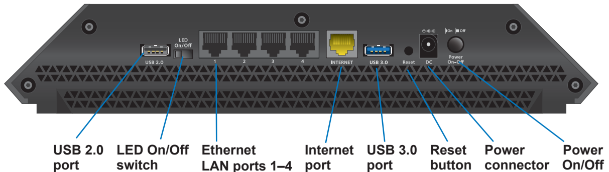
Figure 3. Router rear panel
