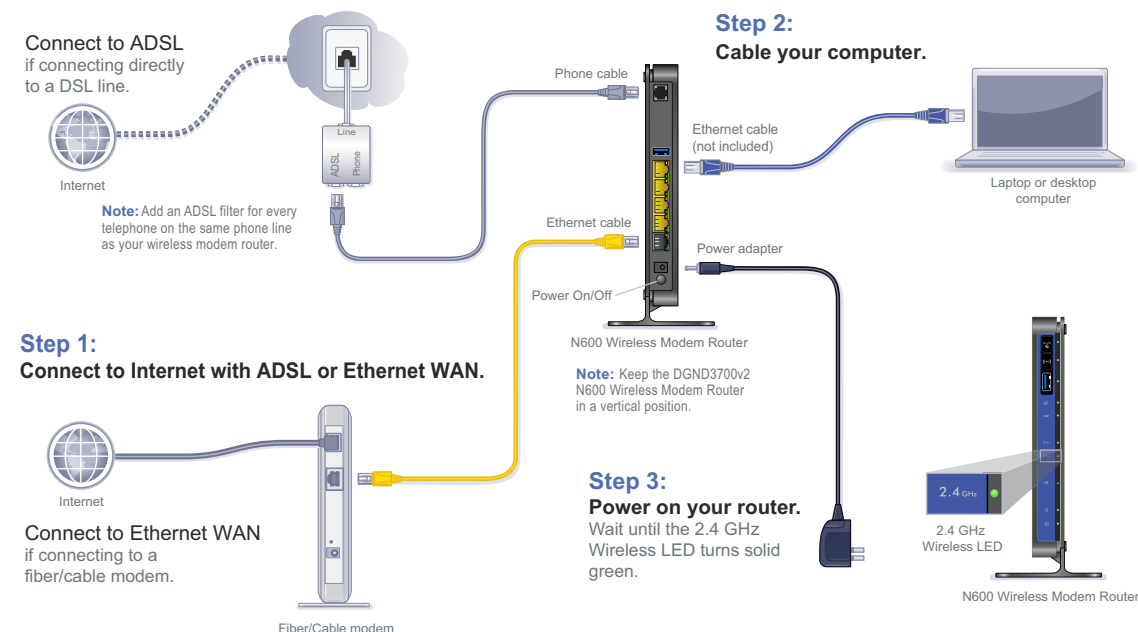
Figure 7. Cabling diagram
