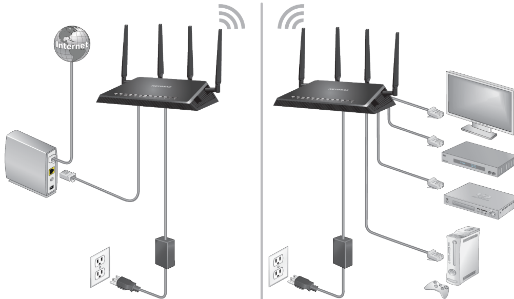
Figure 15. Bridge mode setup with an 802.11ac WiFi connection
