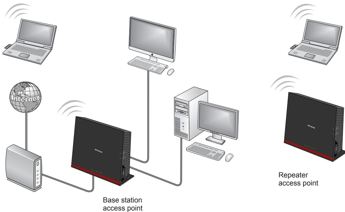
Figure 12. Wireless repeating scenario
