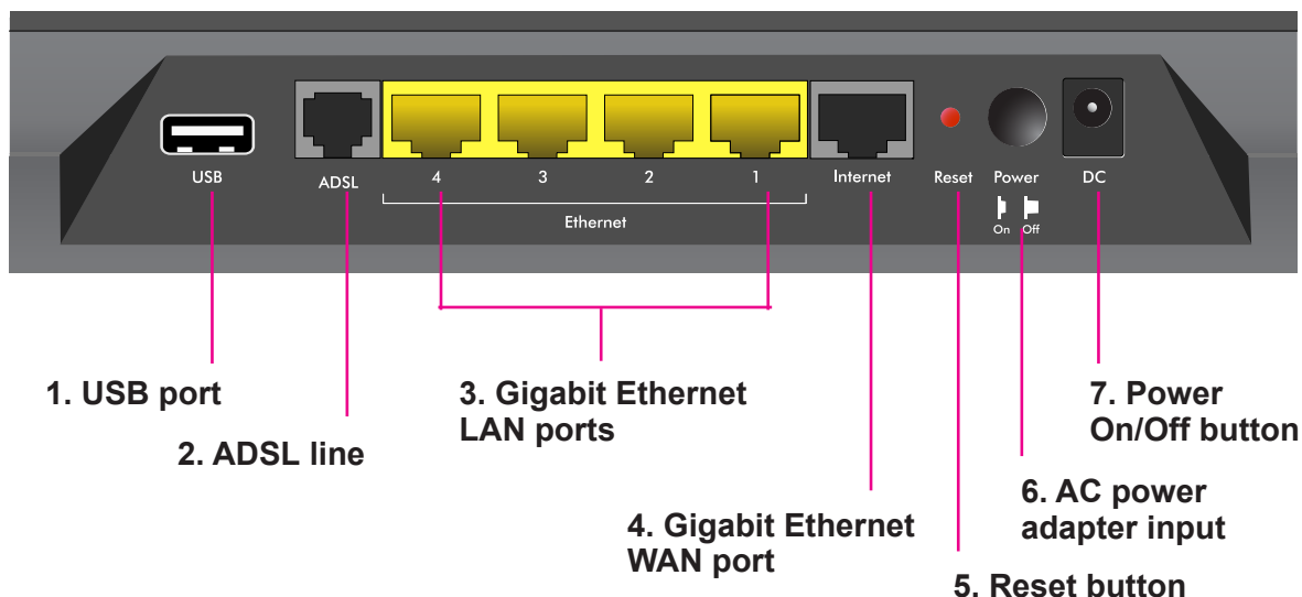
Figure 3. Back panel port connections
