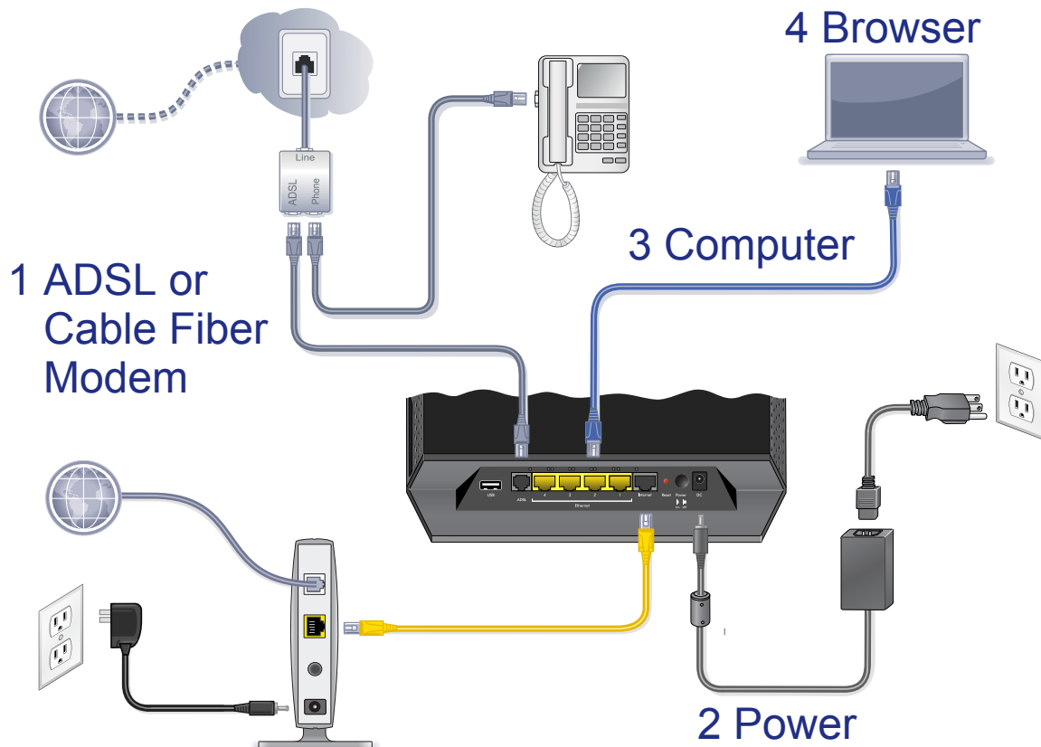
Figure 8. Cabling diagram
