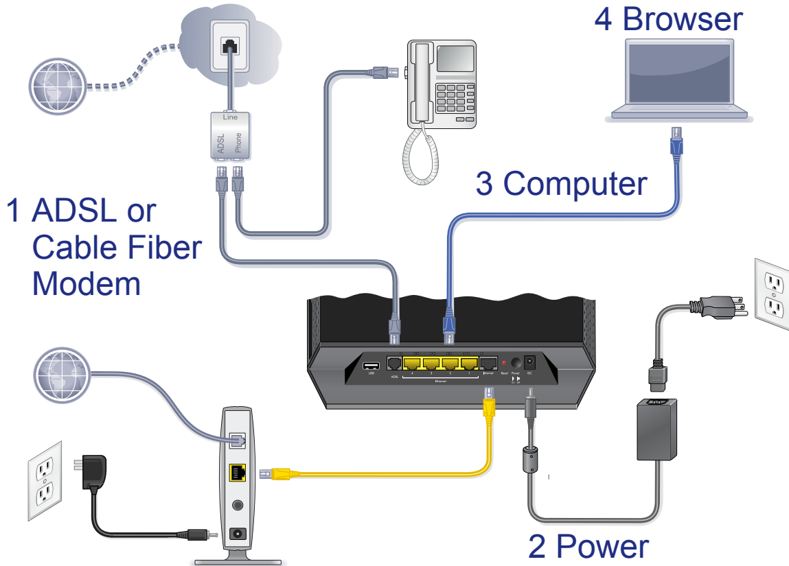
Figure 8. Cabling diagram
