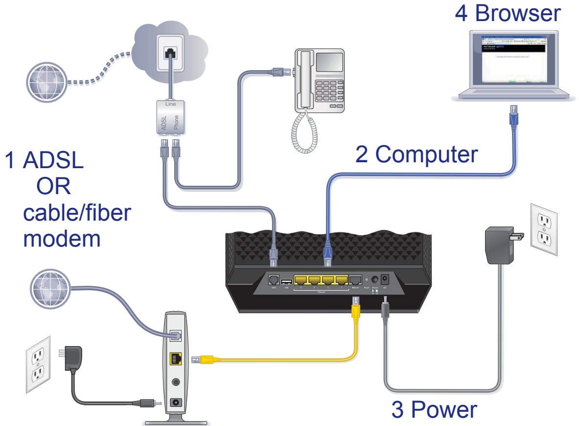
Figure 8. Cabling diagram
